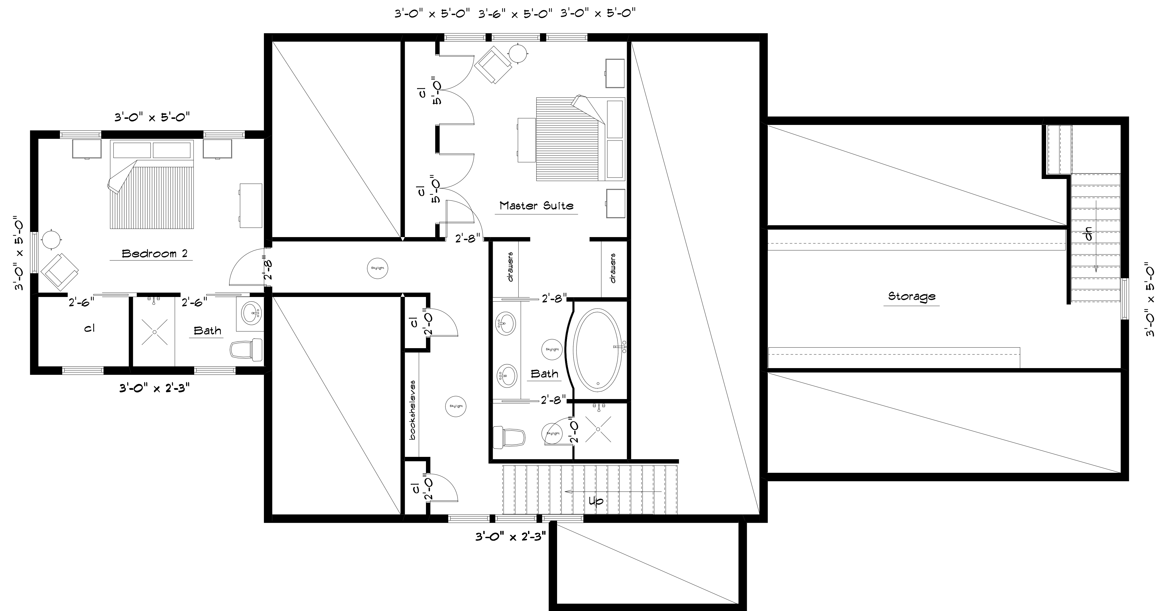
Bungalow Tidewater Second Level 930 Square ft.
